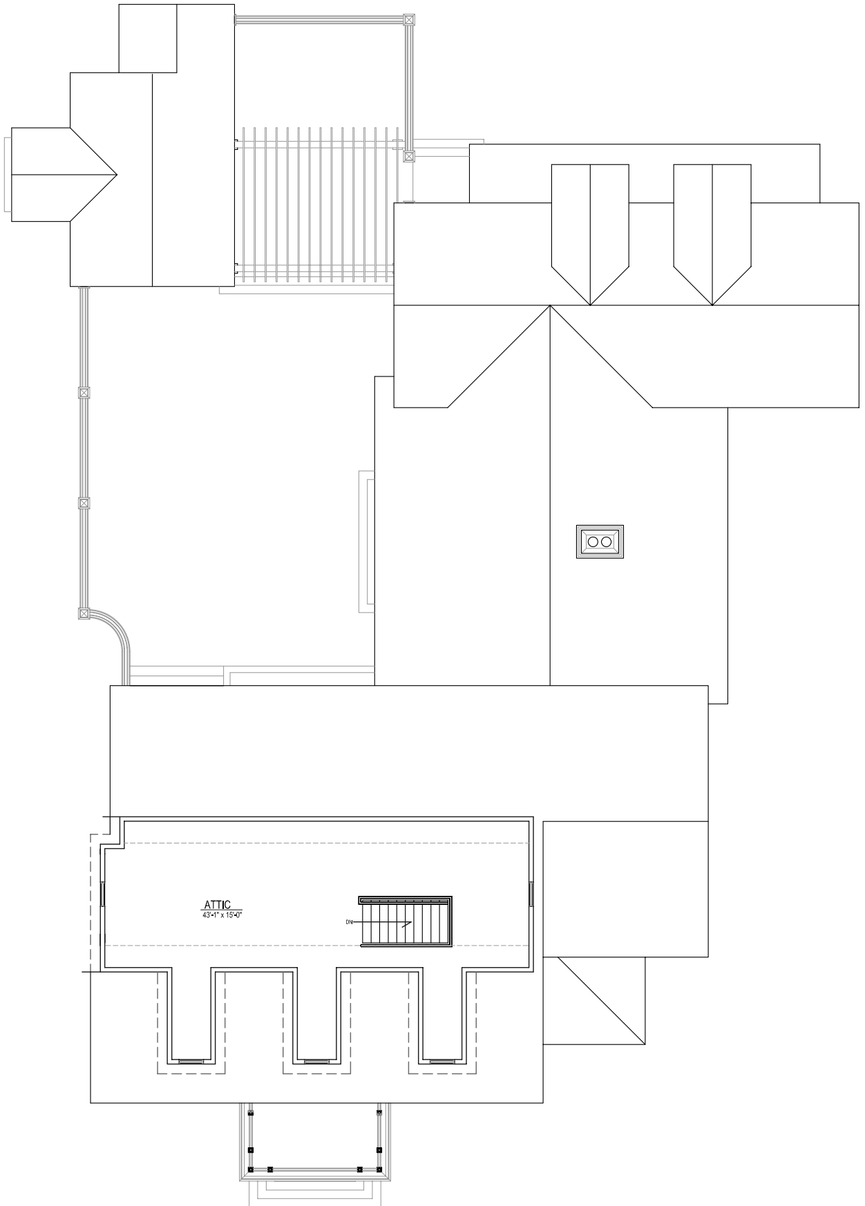
WICKHAM HALL, ATTIC FLOOR PLAN
