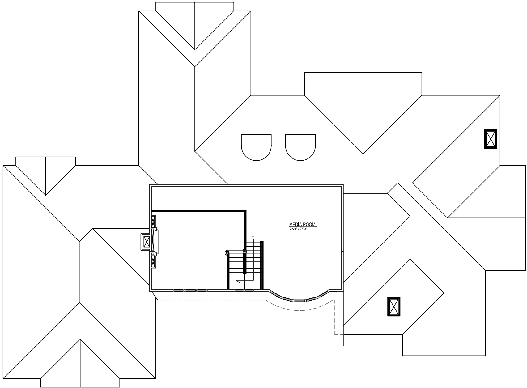
THE PIERPOINTE, SECOND FLOOR PLAN
