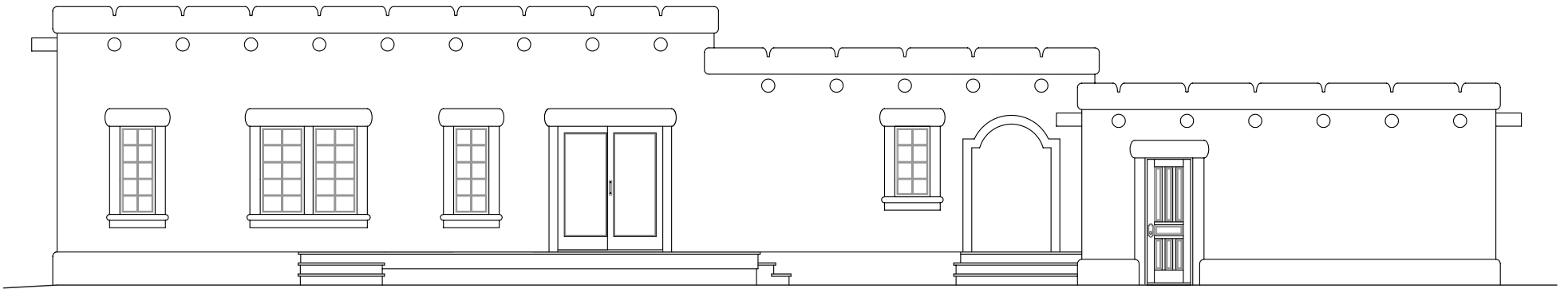
THE OAK (e), REAR ELEVATION (with GARAGE)
