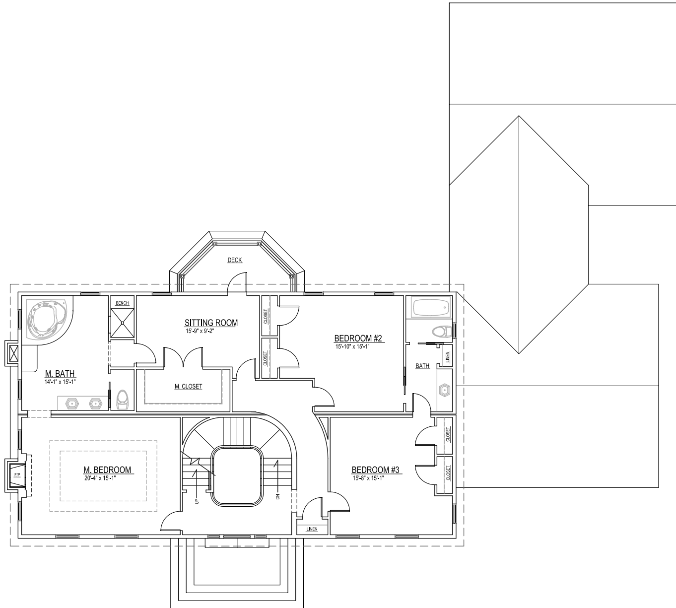
LYME HOUSE, SECOND FLOOR PLAN
