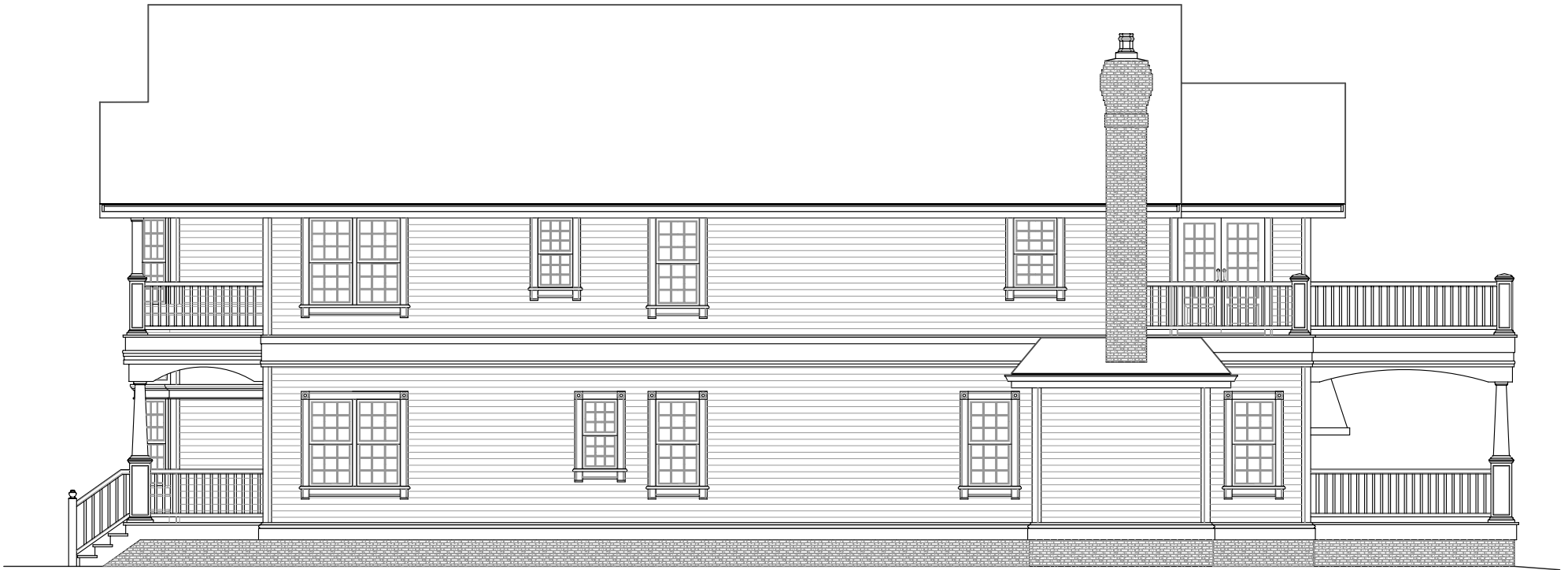
LOUISA COTTAGE, RIGHT ELEVATION, FACING
