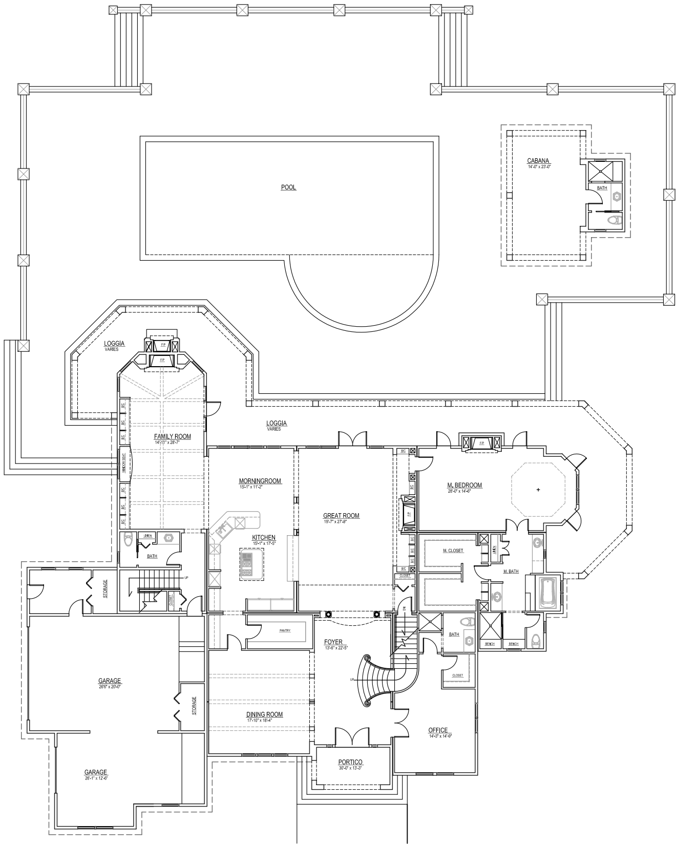
GREUCOEUR 2, FIRST FLOOR PLAN with PATIO and POOL
