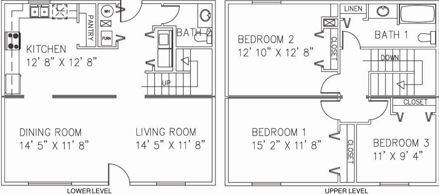
MULTI FAMILY SERIES – TH 3 29' 9" X 25' 9" – 1,528 SQ FT 3 BEDROOMS – 1 1/2 BATHS
