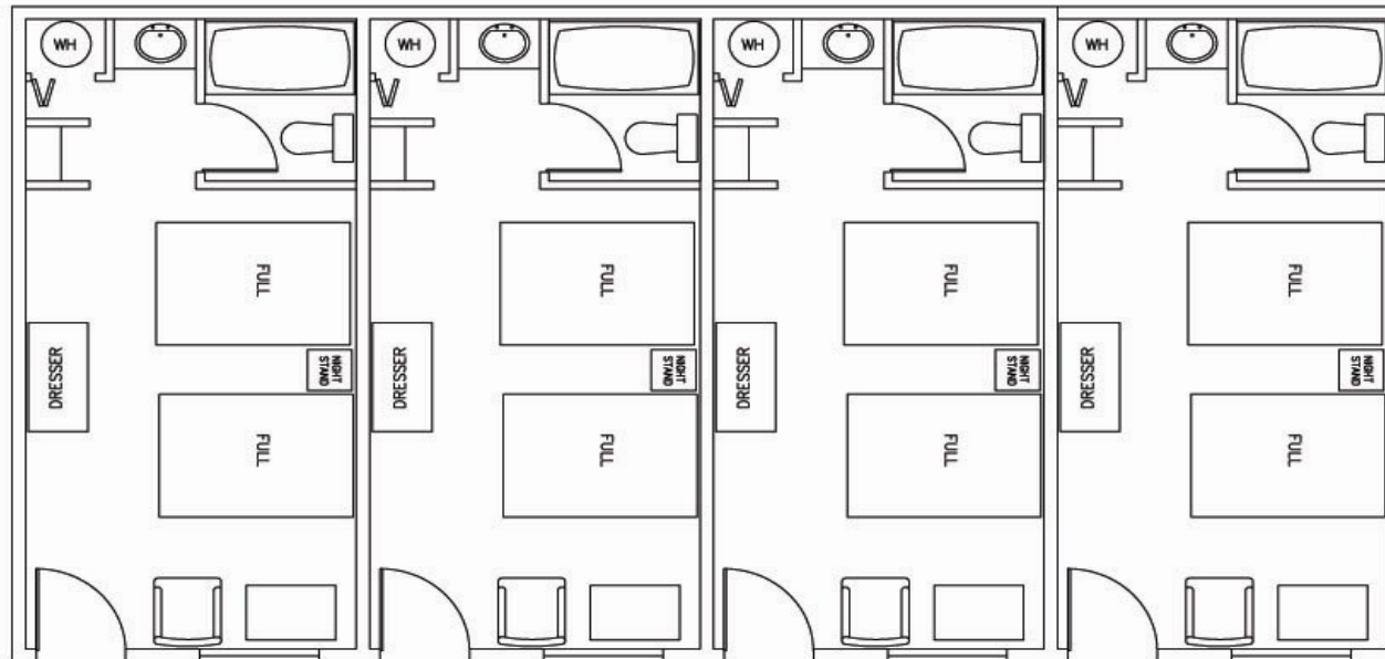
WESTPORT MOTEL 12' X 24' - 208 SQ FT PER UNIT
